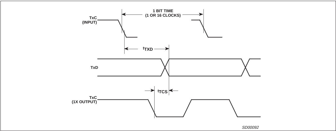
Figure 8. Transmit Timing
